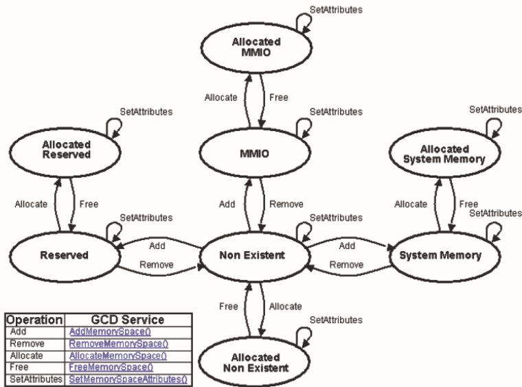
Figure 8.6: GCD Memory State Transitions
