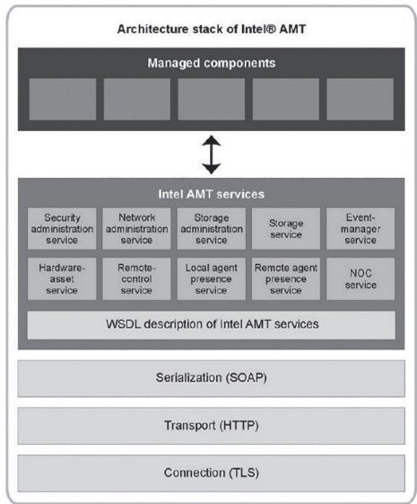
Figure 17.9: Intel® AMT Architecture Stack
