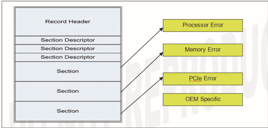
Figure 17.6: UEFI Standard Error Record Format
