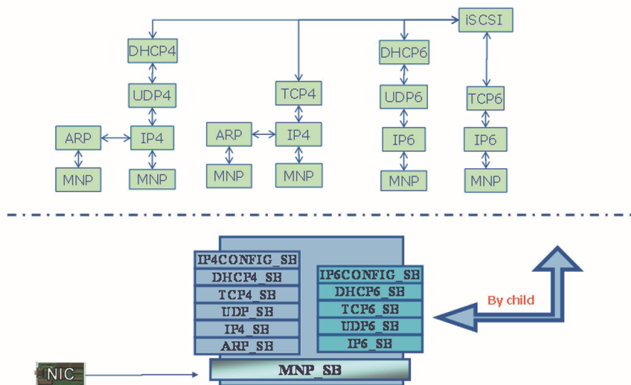
Figure 10.18: An iSCSI Application with UEFI Network Stack
