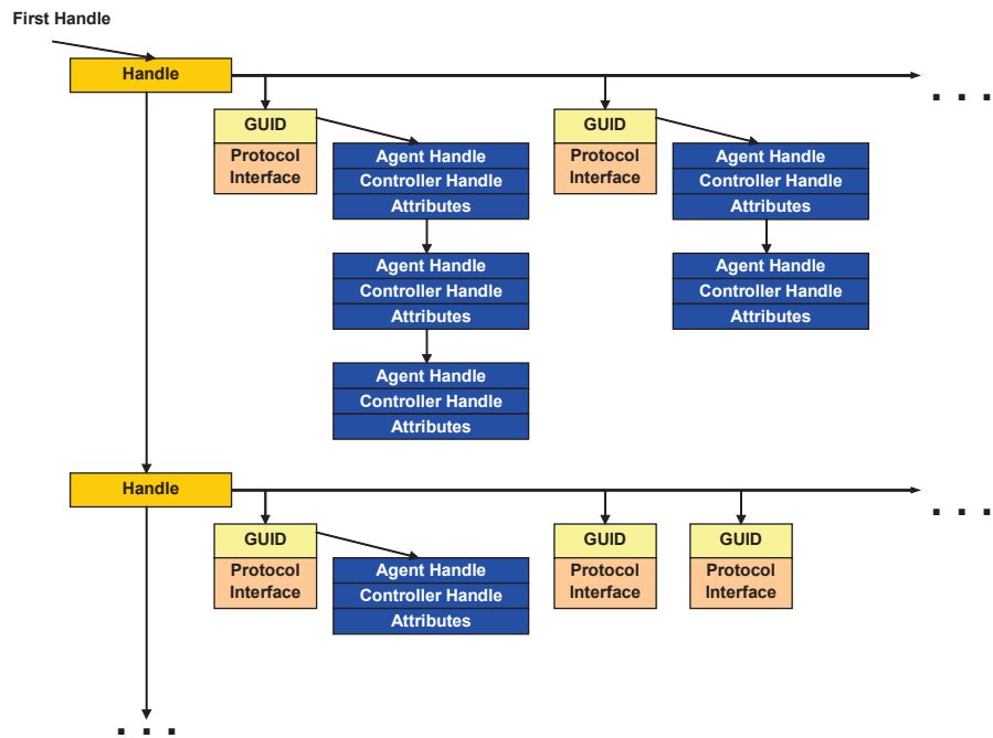
Figure 2.1: Handle Database
