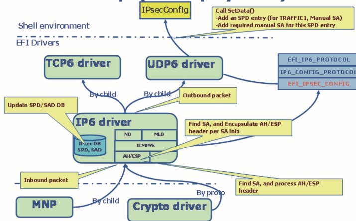
Figure 10.17: UEFI IPsec
