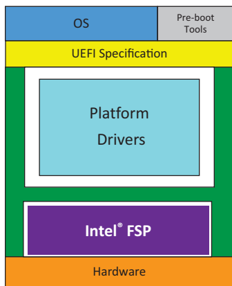
Figure 7.17: Intel ® FSP
