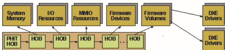
Figure 8.3: HOB List
