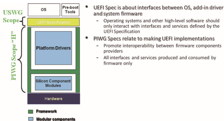
Figure 1.5: PI/UEFI layering
