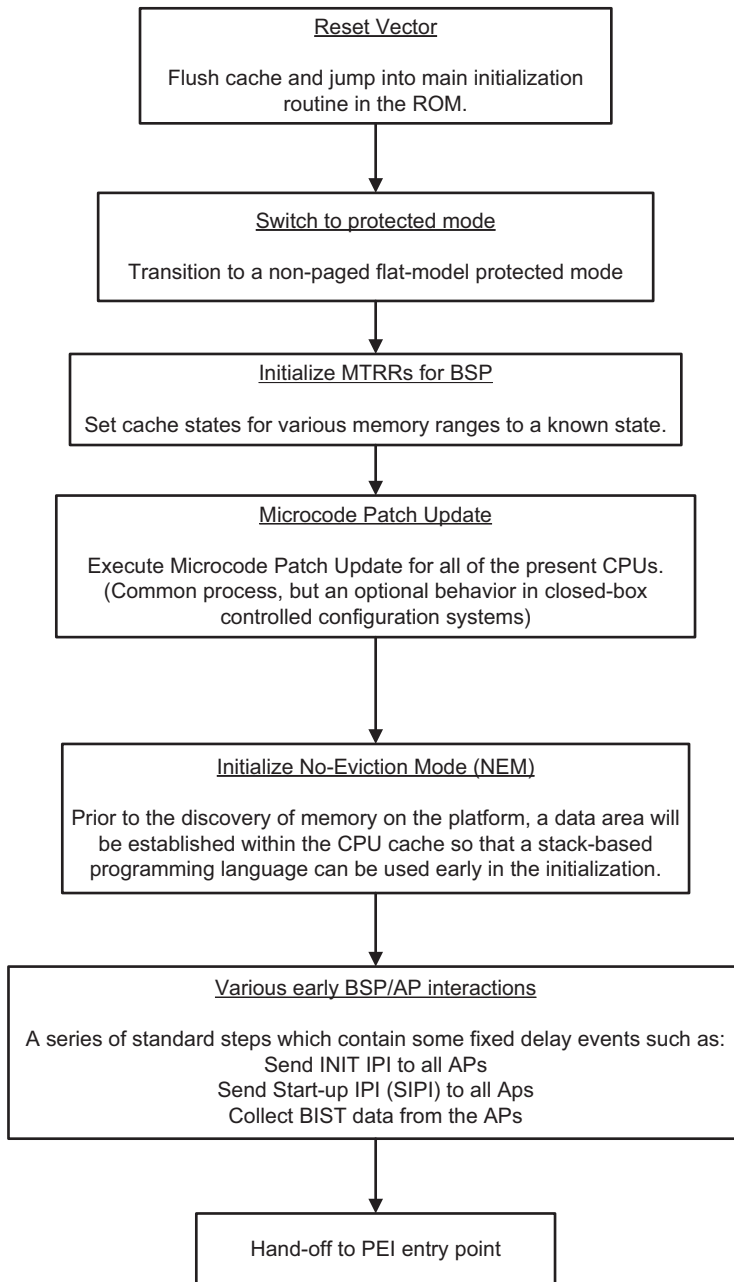
Figure 15.1: SEC Phase
