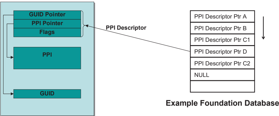
Figure 13.4: How a PPI Is Registered
