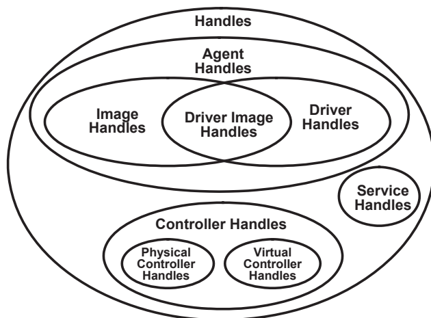
Figure 2.2: Handle Types Handle
