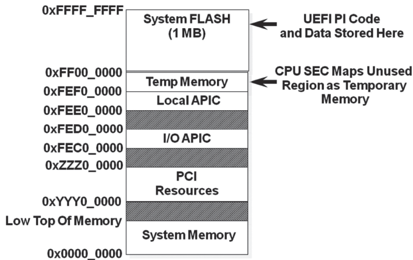
Figure 7.2: System Address Map
