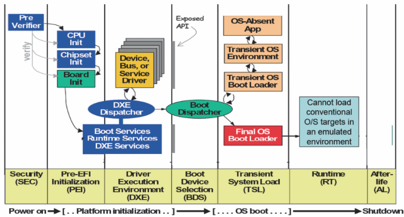
Figure 14.3: The Firmware Emulation Environment Itself
