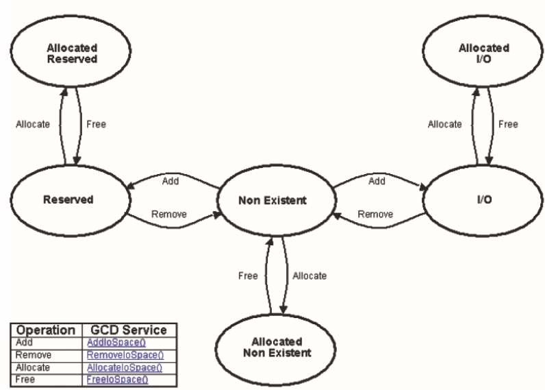
Figure 8.7: GCD I/O State Transitions
