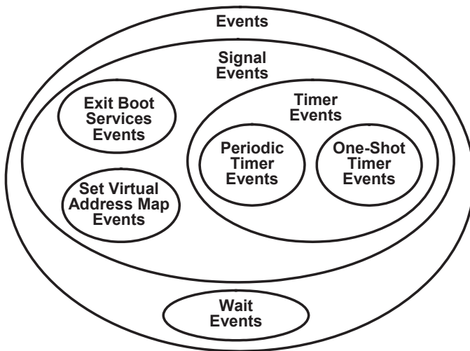
Figure 2.5: Event Types and Relationships
