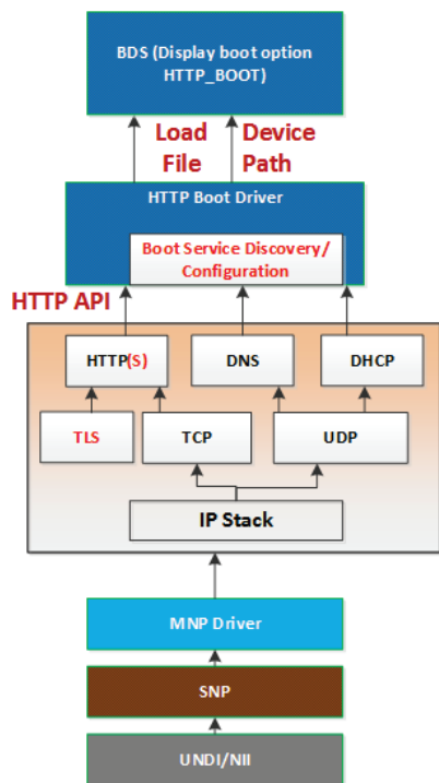
Figure 3.10: HTTP software stack
