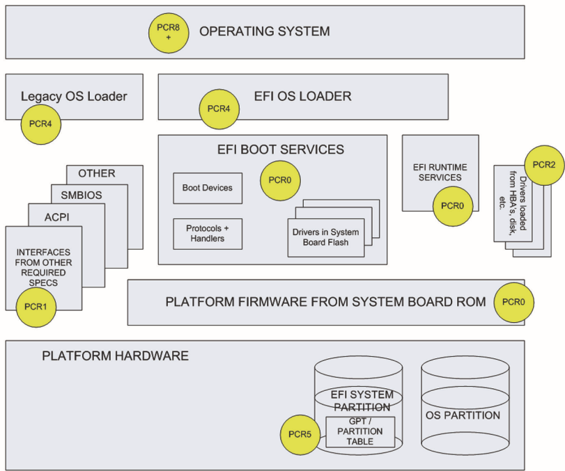
Figure 10.10: Measured Objects in UEFI
