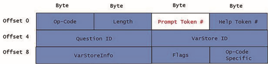
Figure 17.12: Sample IFR Op-code encoding
