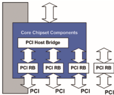
Figure 9.6: Server System with Four PCI Root Bridges
