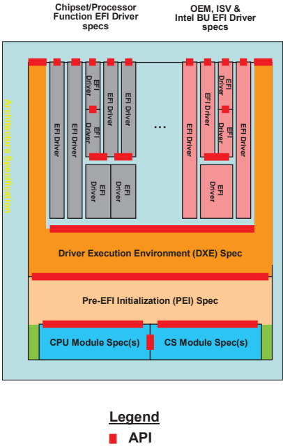
Figure 13.2: System Components
