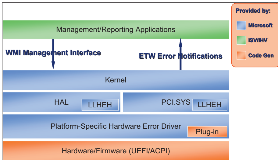
Figure 17.5: WHEA Overview
