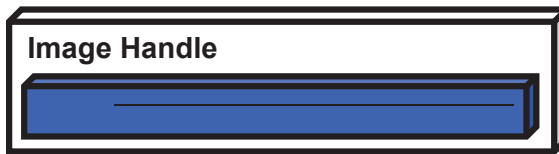
Figure 3.1: Image Handle
