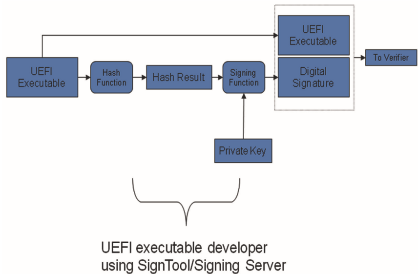
Figure 10.14: Driver signing
