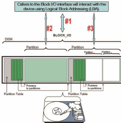
Fig. 9: Software Layering of the Storage Device
