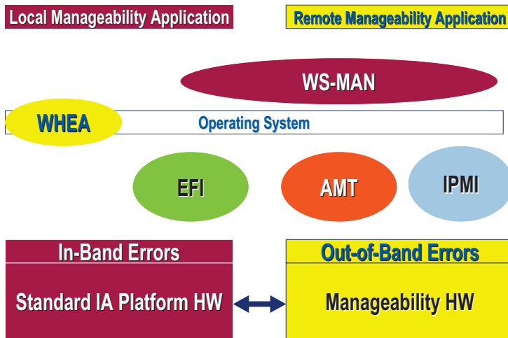
Figure 17.1: Manageability Domains
