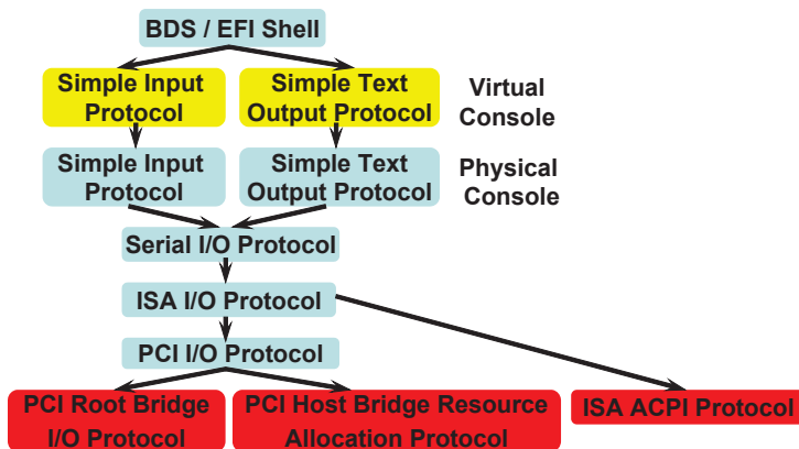
Figure 7.12: Console Stack on a PC
